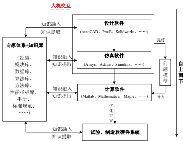
图 1 智能设计与制造平台中各部分间的关系图 Fig.1 The relationship between the components of the intelligent design and manufacturing platform
