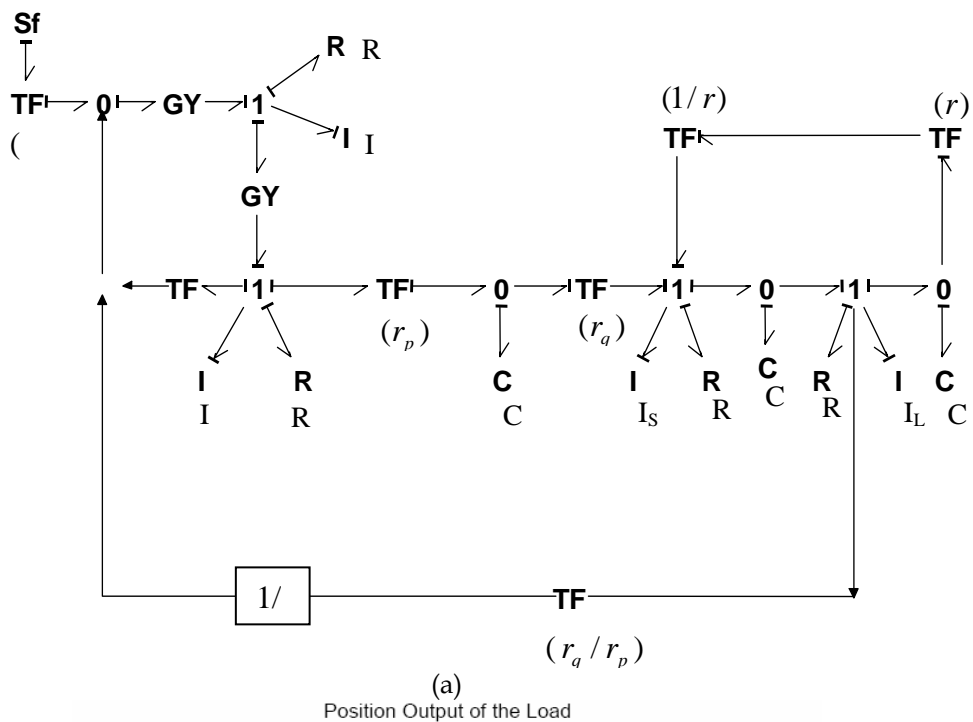
Figure 7. Schematic of the typewriter drive system
