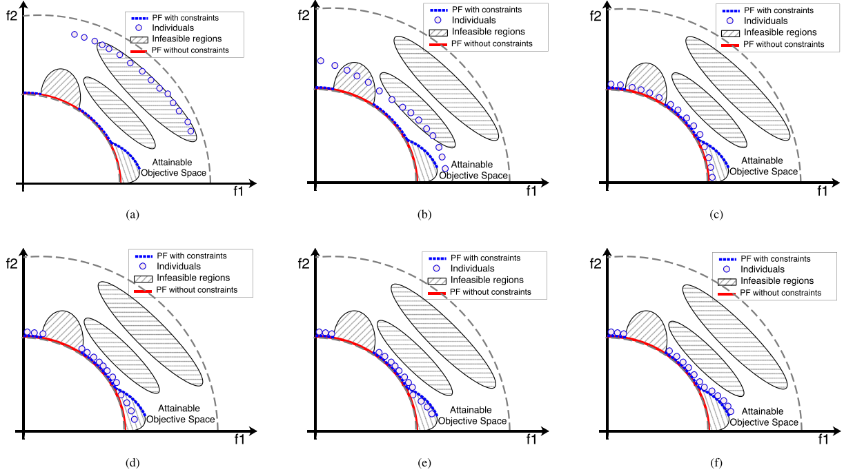
Fig. 3. Infeasible regions make the original unconstrained PF partially feasible. (a)–(c) show the push search process, and some parts of the true PF have been found in this process. In the pull stage, infeasible solutions are gradually pulled to the feasible and non-dominated regions, as shown in (d)–(f).
