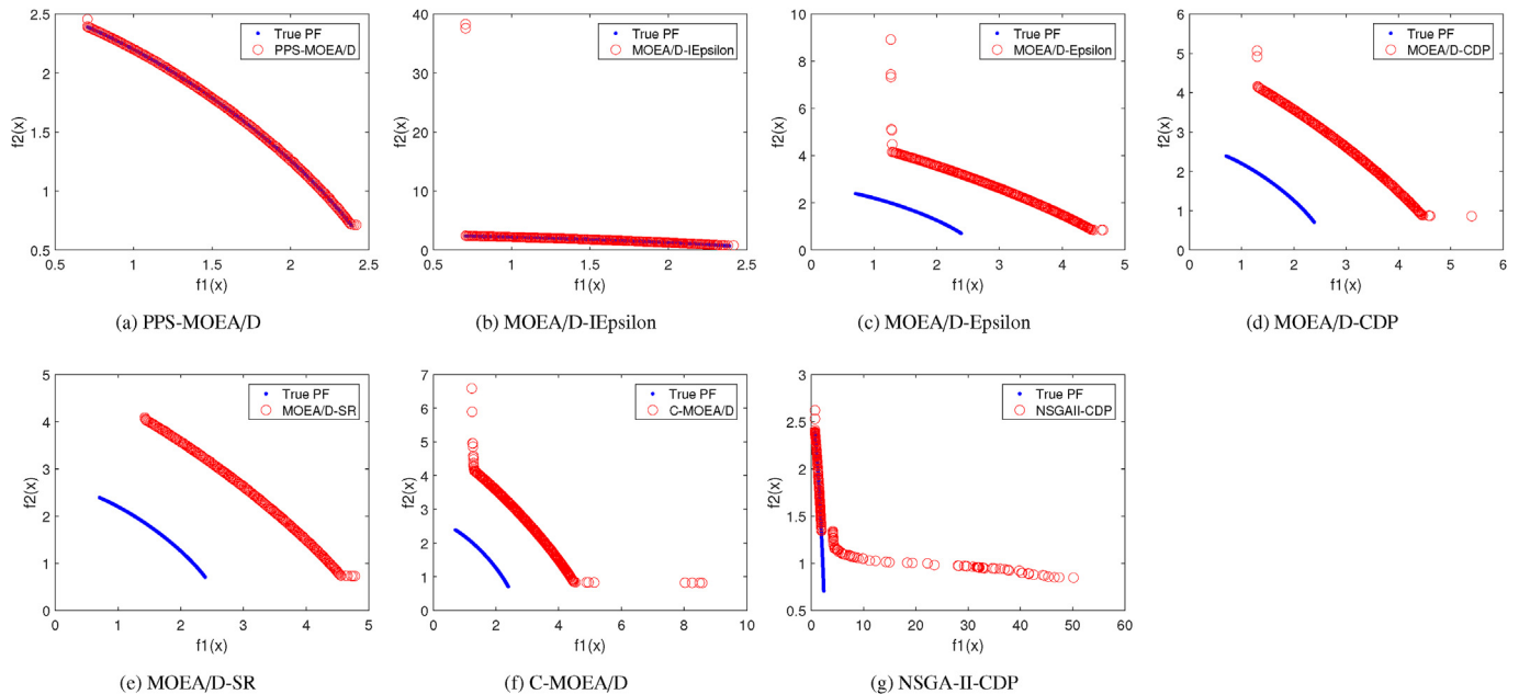
Fig. 6. The non-dominated solutions achieved by each algorithm on LIR-CMOP7 with the median HV values.
