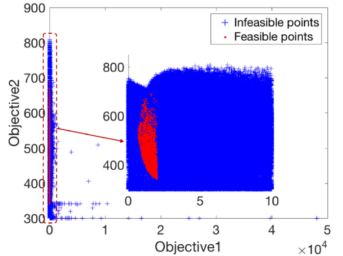
Fig. 9. The distribution of solutions of the robot gripper optimization problem in the objective space.
