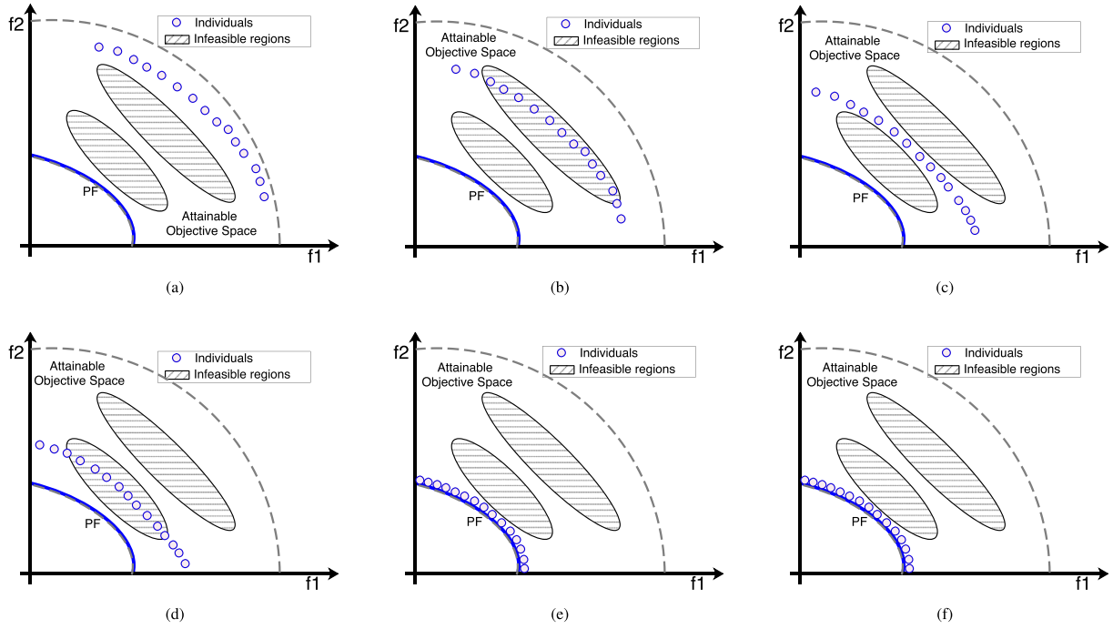
Fig. 1. Infeasible regions block the way towards the PF, and the unconstrained PF is the same as the constrained PF. (a)–(e) show the various stages of the push search process, and show the working population getting across the infeasible regions without any extra efforts dealing with constraints. (f) shows the pull search process, which is the same as (e) in this particular case, since the true PF is the same as the unconstrained PF, and has already been achieved by the working population in the push search process.
