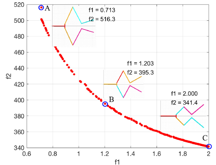
Fig. 11. The non-dominated solutions achieved by PPS-MOEA/D with the best HV value in the 30 independent runs.
