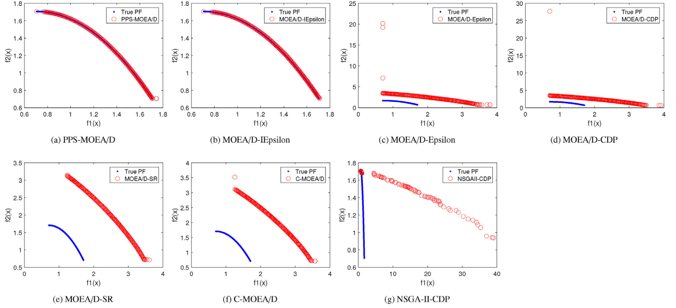
Fig. 5. The non-dominated solutions achieved by each algorithm on LIR-CMOP6 with the median HV values.
