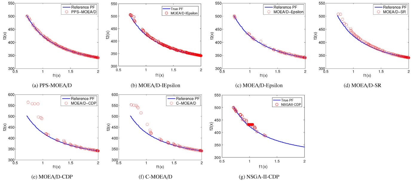
Fig. 10. The non-dominated solutions achieved by each algorithm on the robot gripper optimization problem with the median HV values are plotted in (a)–(g). The reference PF consists of the non-dominated solutions achieved by each algorithm.
