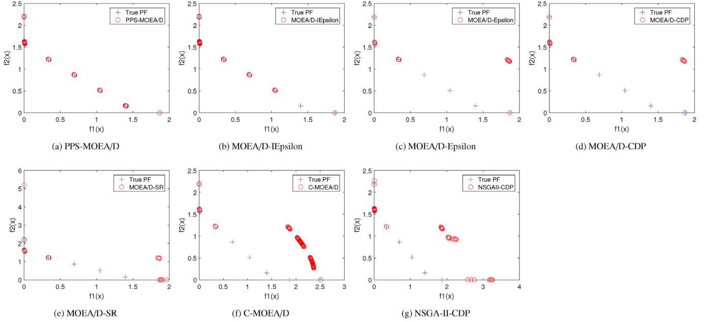
Fig. 7. The non-dominated solutions achieved by each algorithm on LIR-CMOP11 with the median HV values.
