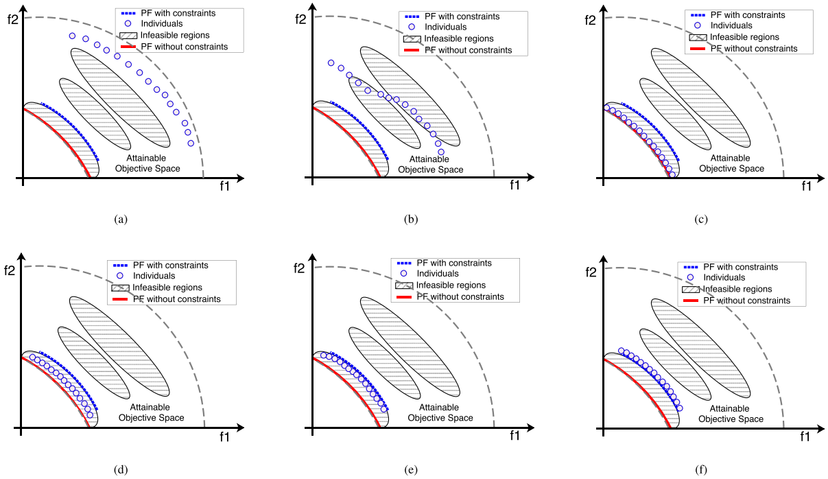
Fig. 2. The unconstrained PF is covered by infeasible regions and all of it is infeasible. The true PF thus lies on some constraint boundaries. (a)–(c) show the push search process, in which the working population crosses the infeasible regions without any barriers. (d)–(f) show the pull search process, in which the infeasible solutions in the working population are gradually pulled to the feasible and non-dominated regions.
