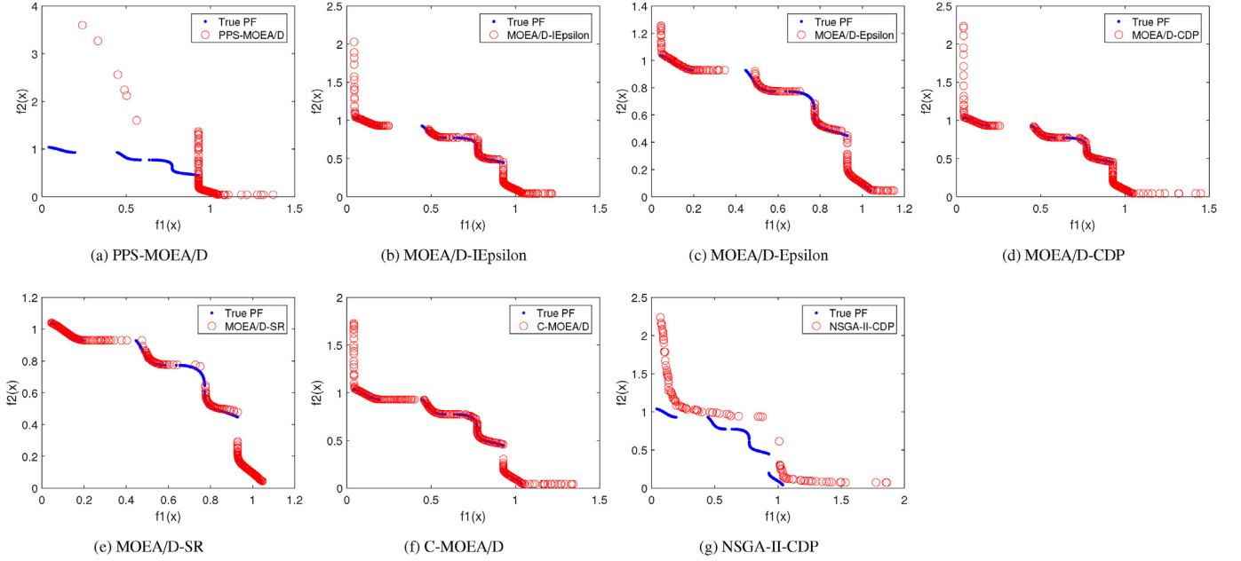
Fig. 8. The non-dominated solutions achieved by each algorithm on TNK-v1 with the median HV values.
