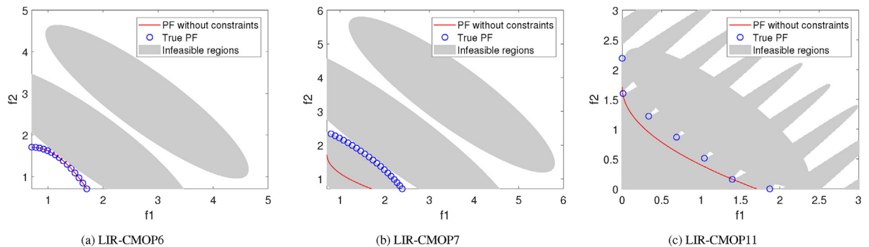
Fig. 4. Illustrations of the feasible and infeasible regions of LIR-CMOP6, LIR-CMOP7 and LIR-CMOP11, corresponding to the three typical situations of infeasible regions influencing PFs as discussed in Section 2.
